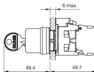
Schlüsselschalter
