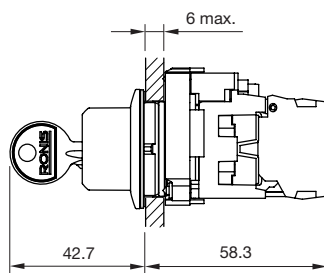
Schlüsselschalter
